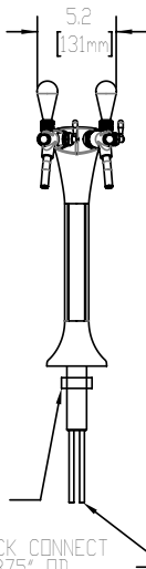
FRONT VIEW
